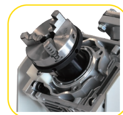
PG-050L Mounts on shaft in replace of table plate
