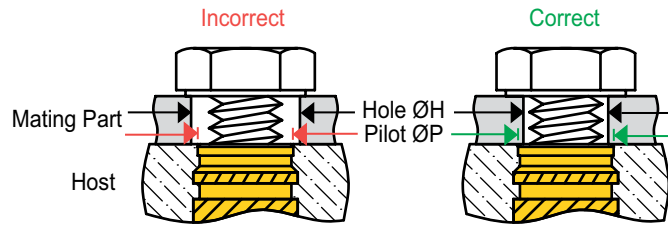
Hole In Mating Part Must Be Smaller Than Insert Pilot Diameter In Host To Prevent The Insert From Pulling Through The Assembly – Known As “Jack-Out”.
