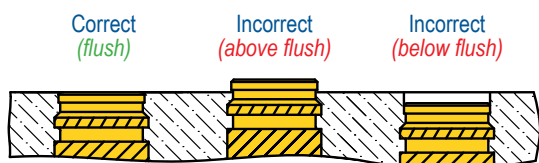
Top of the Insert should be installed as close to flush as possible with the surface of the plastic.
