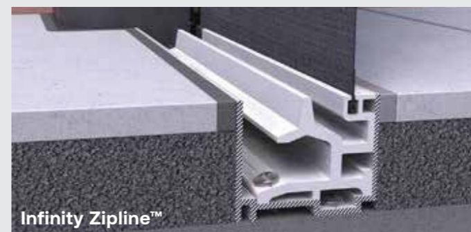
Bottom Track H: 12.5mm W: 63mm Concealed Fixings
