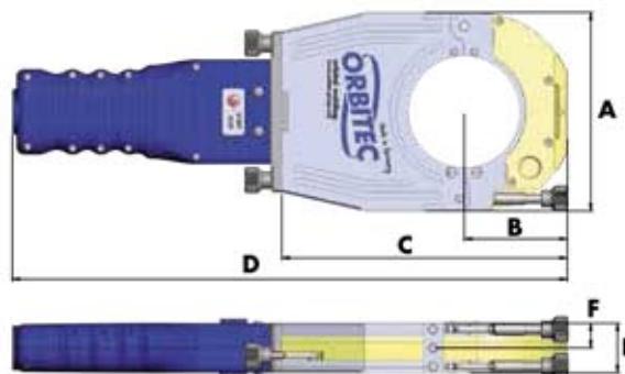
Dimensions table for OSK SW and GW enclosed orbital weld heads
