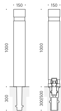
Bollard 057 also available as a lighting bollard (see p. 072: Lighting Bollard 230 LED )
