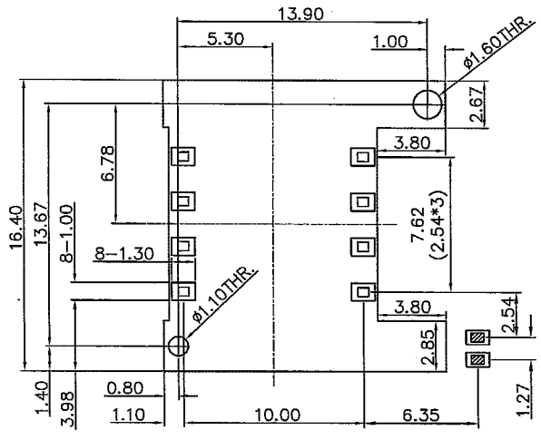
P.C.B. LAYOUT (TOLERANCES:±0.10mm)
